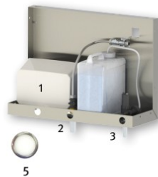
Modular system including high speed hand dryer (1), touch free faucet (2) and liquid soap dispenser (3) and optional lamp soap level indicator (5)
