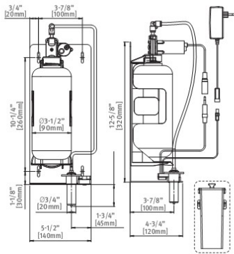
BEHIND MIRROR SD Delivers liquid soap. Battery box for six (6) D batteries/ 12V Transformer PN 280210 - Battery Version PN 280200 - 12V Transformer
