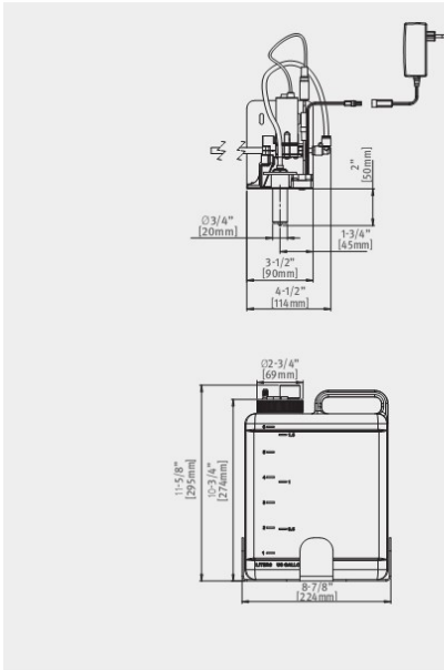
MF BEHIND MIRROR FOAM Soap foam dispenser to be used with Stern's Multifeed kits for multiple refill. Delivers foam soap. PN 07292270
