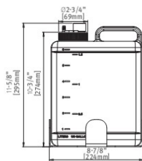
MULTIFEED KIT This version allows multiple soap dispenser refill (up to 6 dispensers) with a single 1.6 US Gallons (6 liters) tank. PN 07220096
