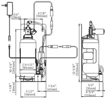
BTM FOAM E Delivers foam soap 12V Transformer PN 280250
