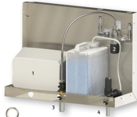
Complete system including high speed hand dryer (1), thermostatic mixing valve (2), touch free faucet (3) liquid soap dispenser (4) and optional lamp soap level indicator (5)
